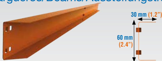
Largero Serie U122 - Beam U122 Series
